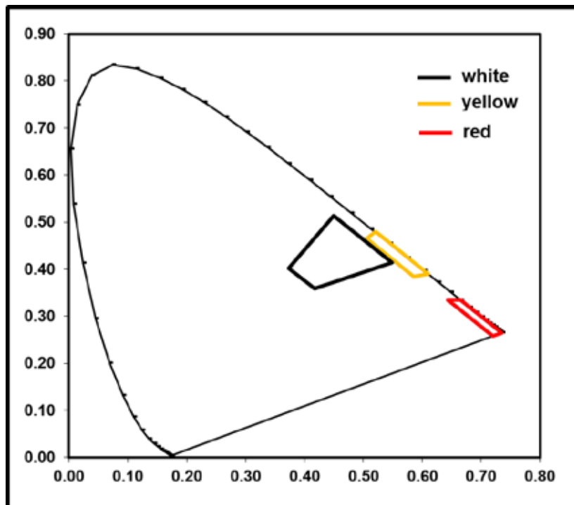
Figure A: CIE Color Diagram
