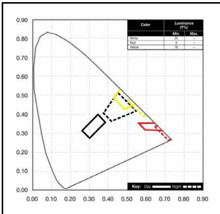
Figure A: CIE Color Diagram
